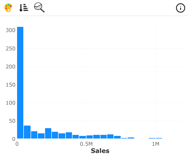
Sales Distribution
